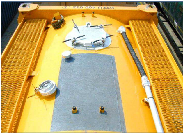
Roof view with walkway and anti-slip surface
